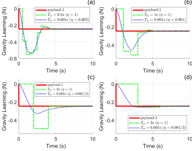
Fig. 2: Simulation results of scaling down the iterative update time ( T_{it} , i.e., the steady-state time) while scaling down the iterative learning rate ( \eta ) accordingly. The reference is an external payload-1 (25g). The setpoint is set as [0.01, 0.04, 0] m in Cartesian space.
