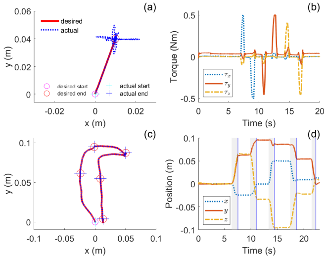
Fig. 10: Experimental results in a setpoint regulation task involving pHRI . (a) Trajectory when pHRI disabled; (b) Computed torque when pHRI disabled; (c) Trajectory when pHRI enabled; (d) Actual position when pHRI enabled. Note, the five shaded areas in (d) indicate five times of interaction during which the user moves the robot EE from one point to another as shown in (c). The five vertical blue lines in (d) are the time points corresponding to the five actual endpoints in (c).
